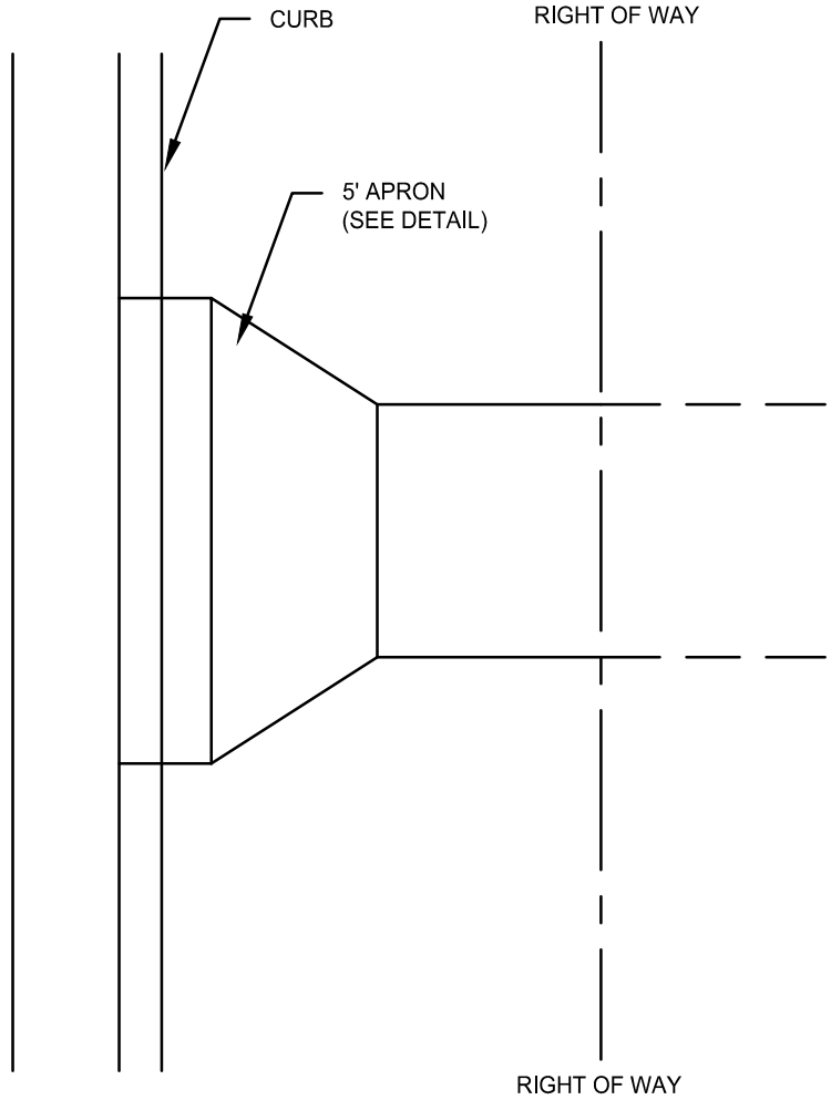
BITUMINOUS DRIVEWAY REPLACEMENT
